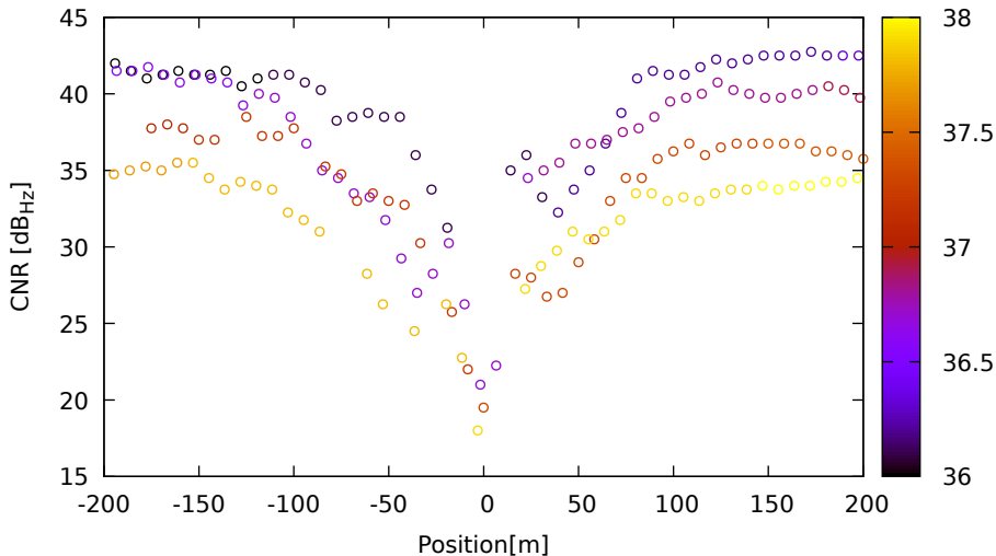
CNR vs position for E11 (E1) on SamsungS20 - DOY 263 jam. 2
