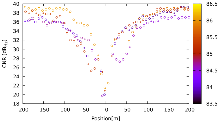
CNR vs position for E12 (E1) on SamsungS20 - DOY 263 jam. 2
