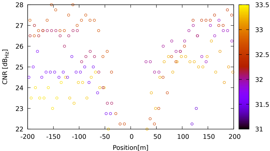
CNR vs position for E33 (E5a) on SamsungS20 - DOY 263 jam. 1
