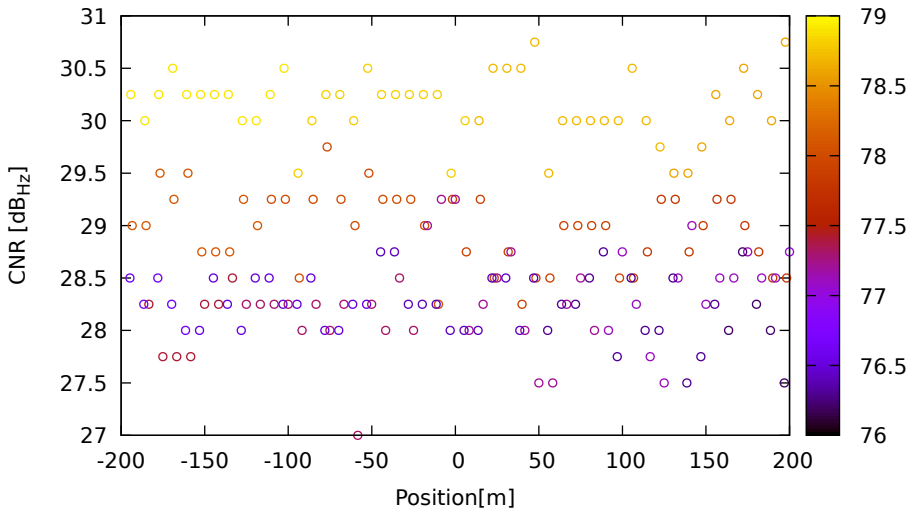
CNR vs position for G01 (L5) on SamsungS20 - DOY 263 jam. 2
