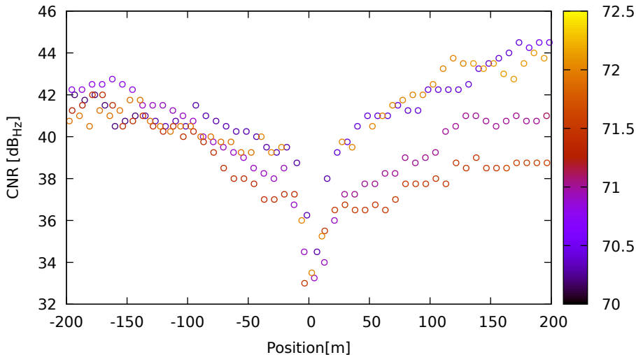
CNR vs position for G03 (L1) on SamsungS20 - DOY 263 jam. 1
