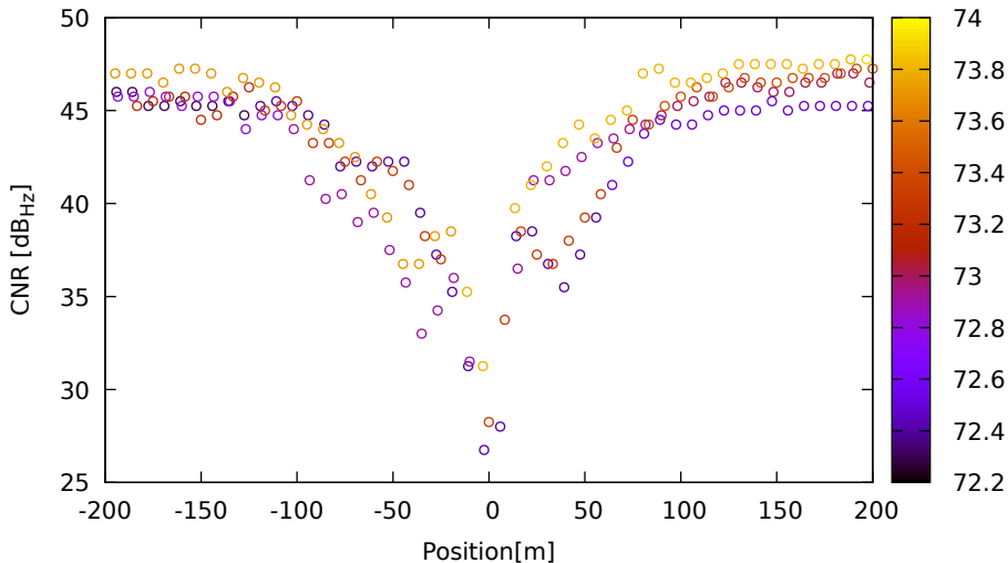
CNR vs position for G03 (L1) on SamsungS20 - DOY 263 jam. 2
