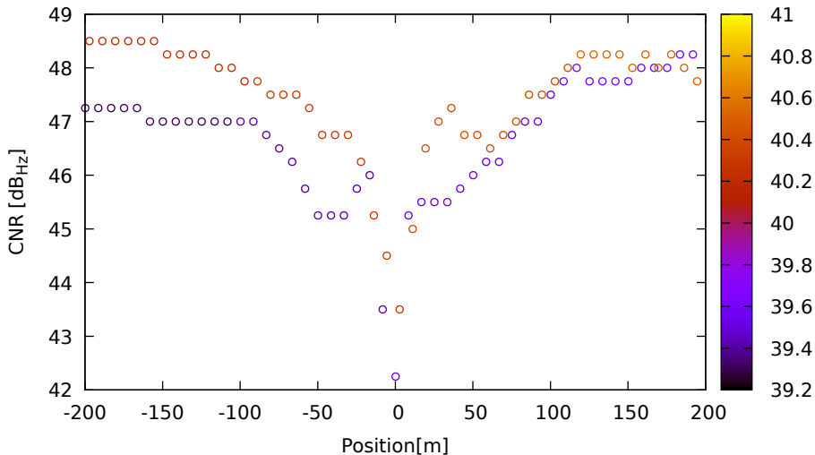
CNR vs position for G04 (L1) on SamsungS20 - DOY 263 jam. 3
