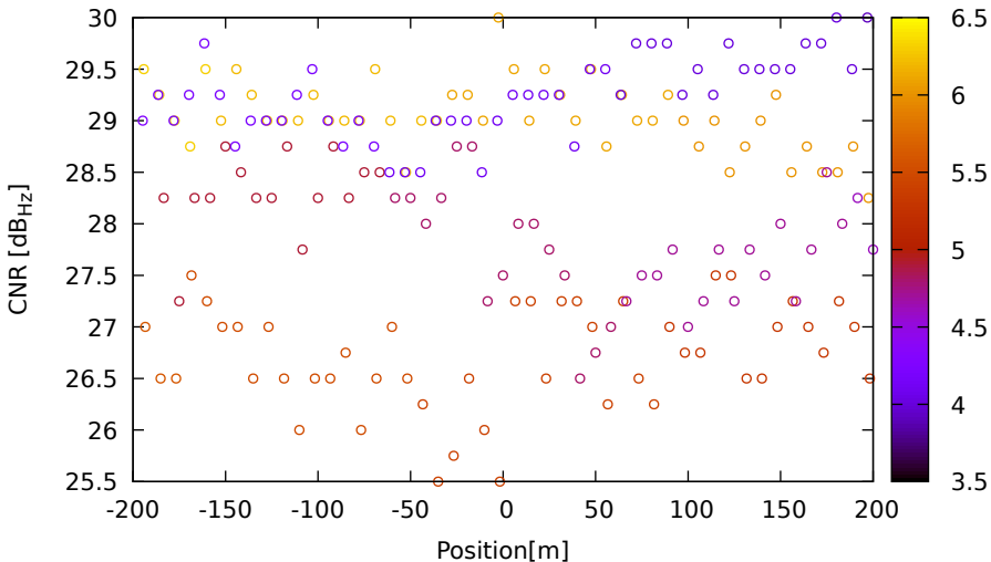
CNR vs position for G08 (L5) on SamsungS20 - DOY 263 jam. 2
