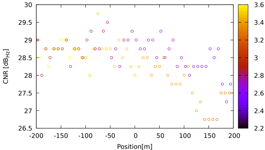
CNR vs position for G08 (L5) on SamsungS20 - DOY 263 jam. 3
