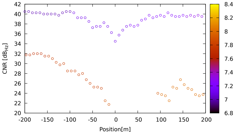
CNR vs position for G09 (L1) on SamsungS20 - DOY 263 jam. 3
