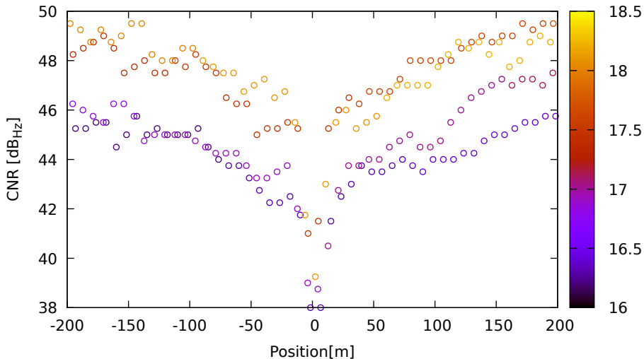
CNR vs position for G19 (L1) on SamsungS20 - DOY 263 jam. 1
