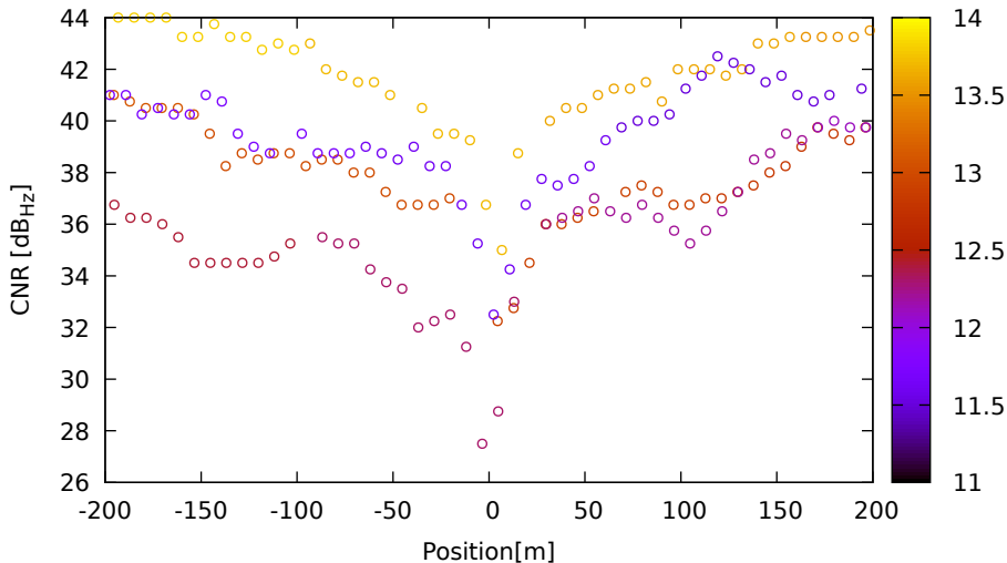
CNR vs position for G32 (L1) on SamsungS20 - DOY 263 jam. 1
