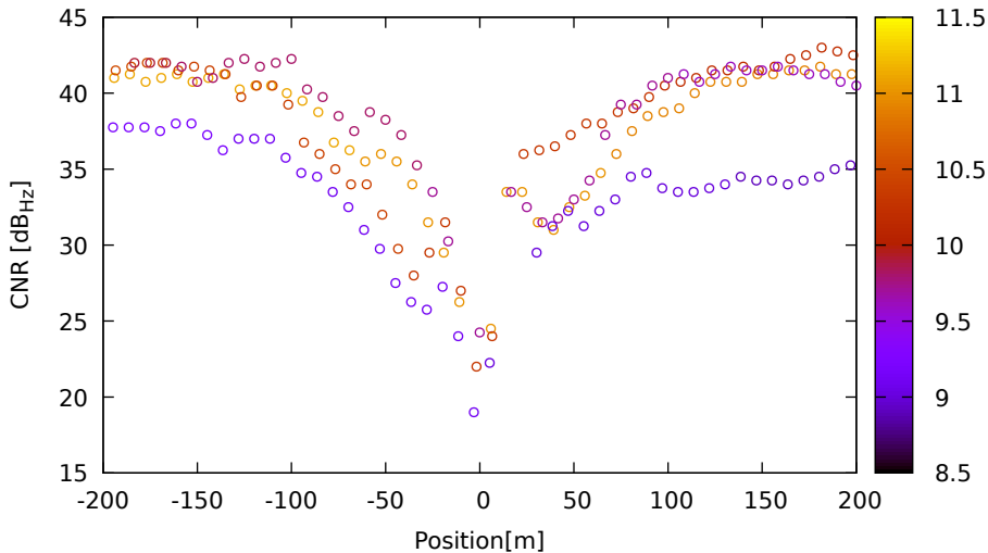
CNR vs position for G32 (L1) on SamsungS20 - DOY 263 jam. 2
