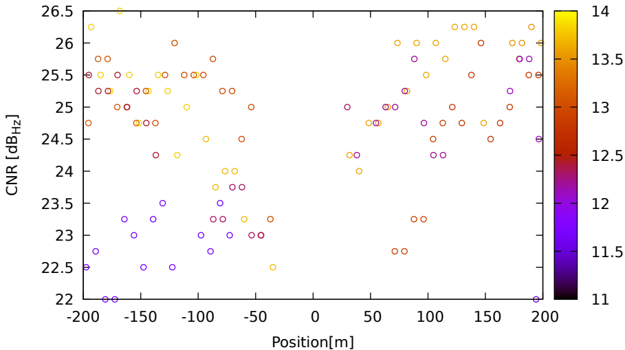
CNR vs position for G32 (L5) on SamsungS20 - DOY 263 jam. 1
