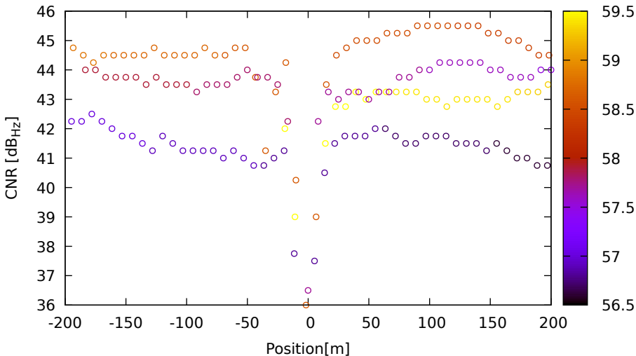
CNR vs position for R01 (G1) on SamsungS20 - DOY 263 jam. 2
