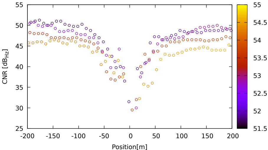
CNR vs position for R02 (G1) on SamsungS20 - DOY 263 jam. 1
