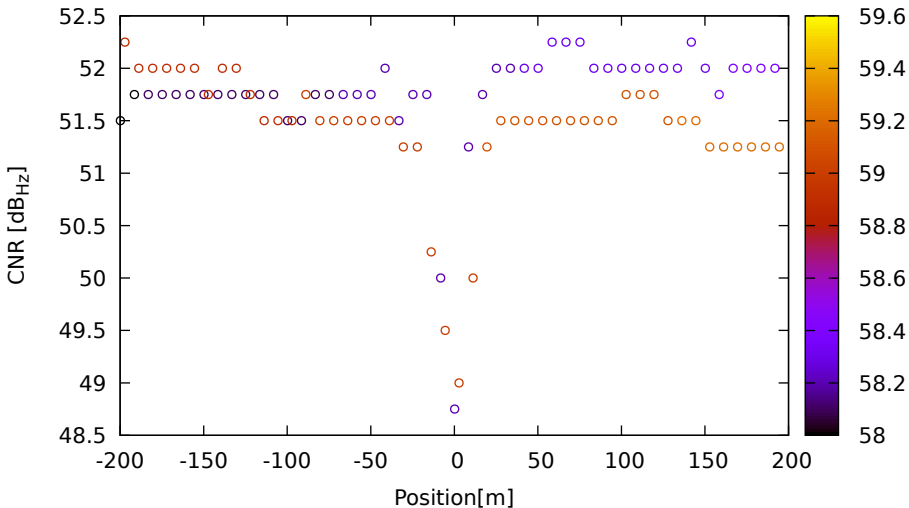
CNR vs position for R02 (G1) on SamsungS20 - DOY 263 jam. 3
