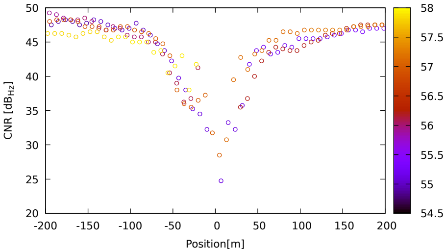
CNR vs position for R17 (G1) on SamsungS20 - DOY 263 jam. 1
