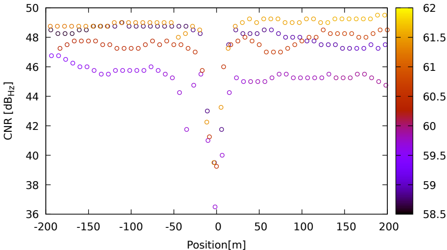
CNR vs position for R17 (G1) on SamsungS20 - DOY 263 jam. 2
