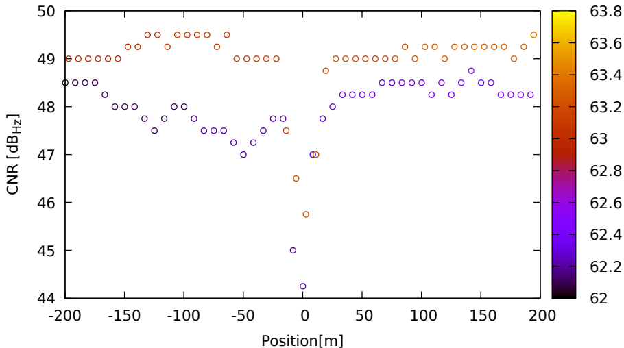
CNR vs position for R17 (G1) on SamsungS20 - DOY 263 jam. 3
