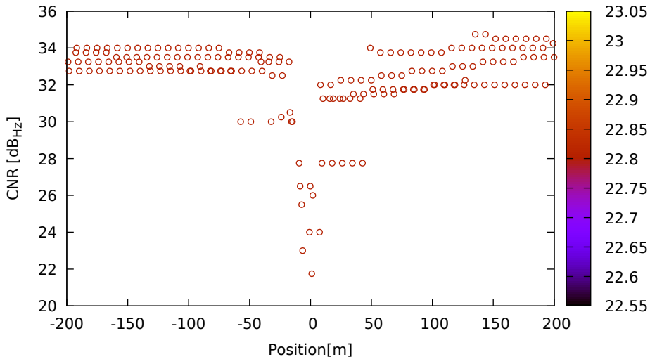
CNR vs position for C05 (B1) on Xiaomi11T - DOY 263 jam. 1
