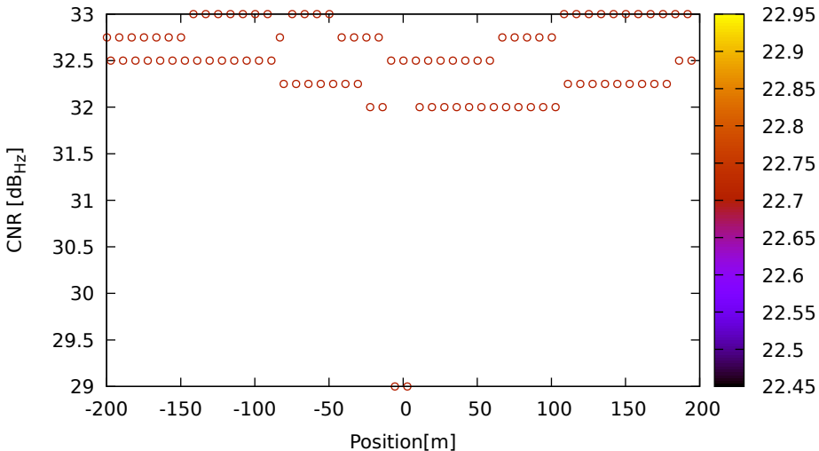
CNR vs position for C05 (B1) on Xiaomi11T - DOY 263 jam. 3
