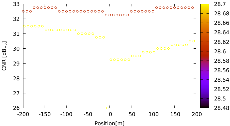
CNR vs position for C06 (B1) on Xiaomi11T - DOY 263 jam. 3
