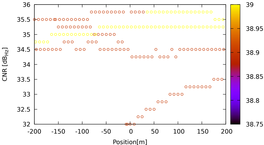
CNR vs position for C09 (B1) on Xiaomi11T - DOY 263 jam. 2
