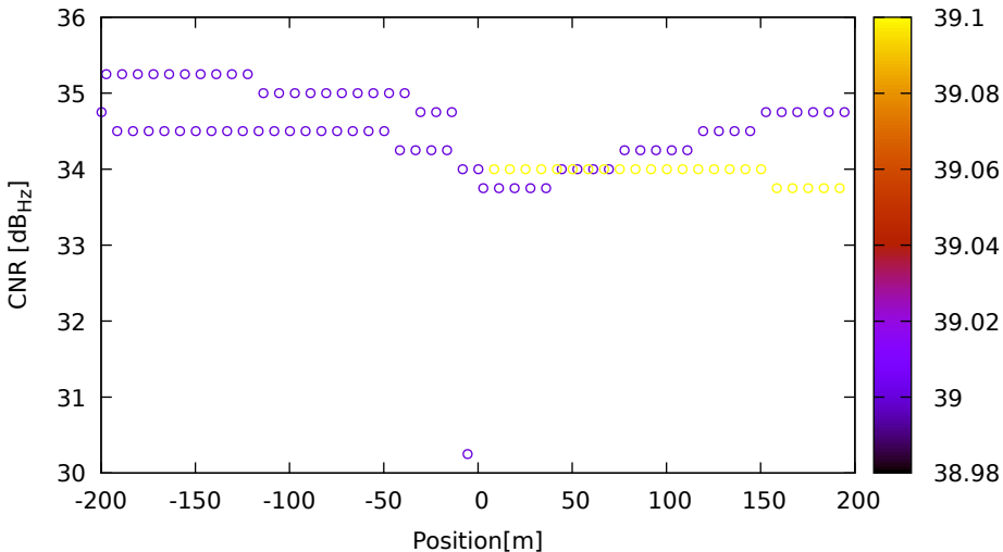
CNR vs position for C09 (B1) on Xiaomi11T - DOY 263 jam. 3
