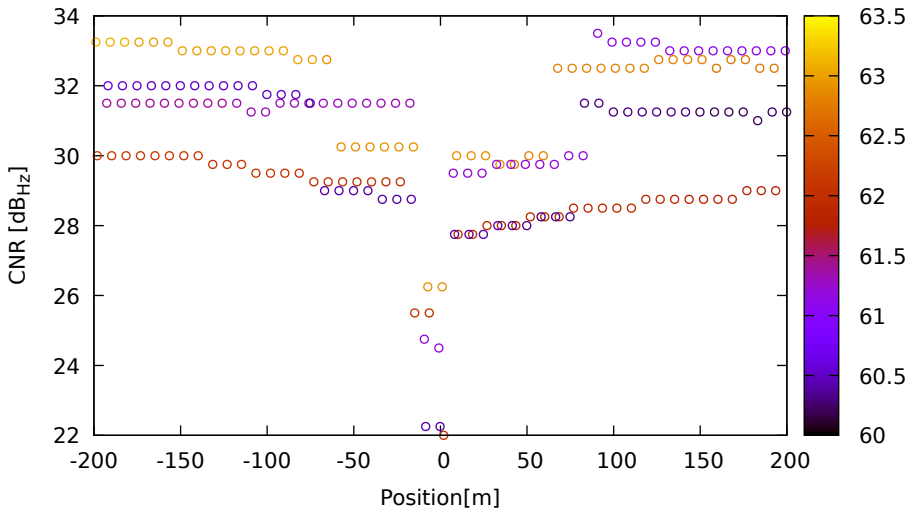
CNR vs position for C11 (B1) on Xiaomi11T - DOY 263 jam. 1
