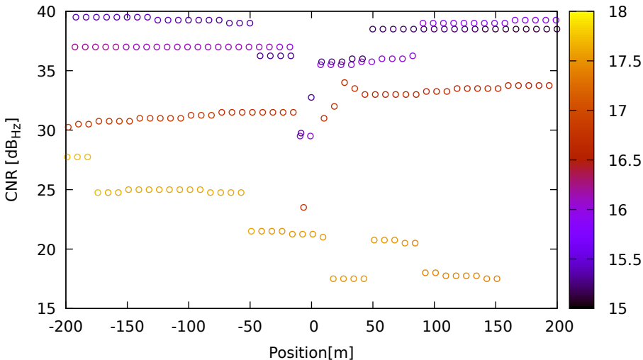
CNR vs position for C12 (B1) on Xiaomi11T - DOY 263 jam. 1
