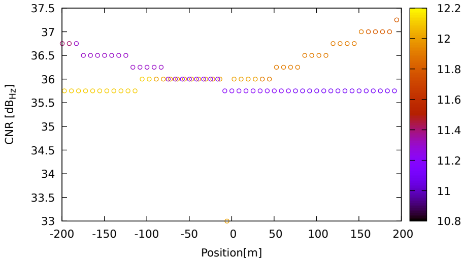
CNR vs position for C12 (B1) on Xiaomi11T - DOY 263 jam. 3
