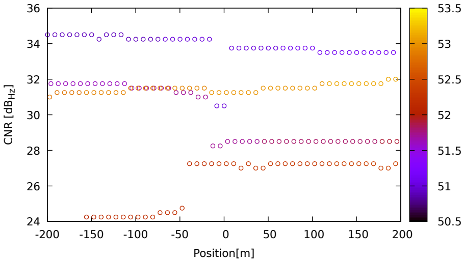
CNR vs position for C14 (B1) on Xiaomi11T - DOY 263 jam. 2
