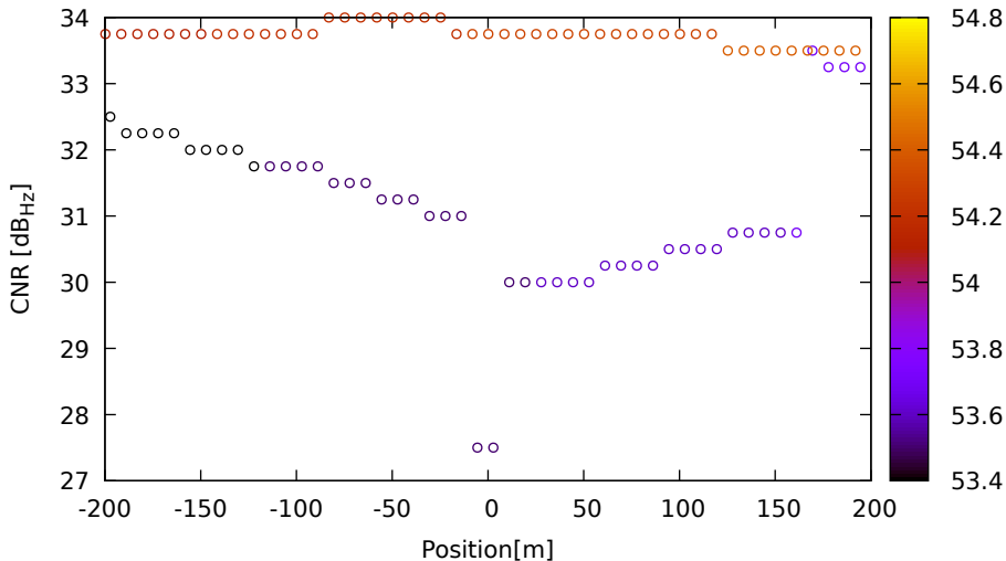
CNR vs position for C14 (B1) on Xiaomi11T - DOY 263 jam. 3
