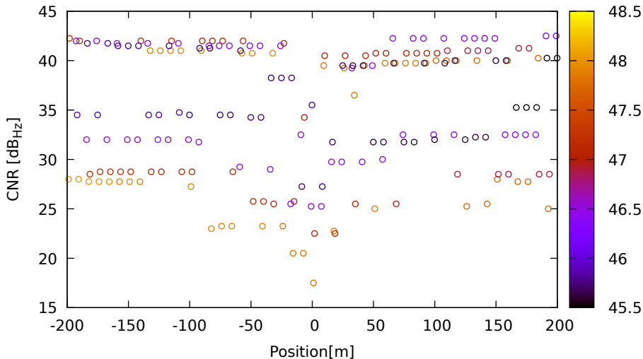
CNR vs position for C21 (B1) on Xiaomi11T - DOY 263 jam. 1
