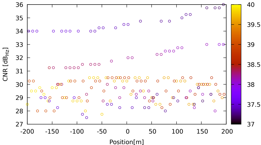
CNR vs position for C34 (B1) on Xiaomi11T - DOY 263 jam. 2
