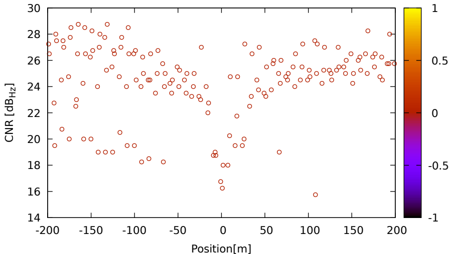
CNR vs position for E02 (E1) on Xiaomi11T - DOY 263 jam. 1
