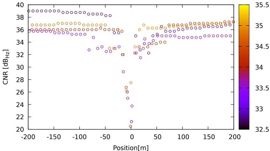
CNR vs position for E04 (E1) on Xiaomi11T - DOY 263 jam. 1
