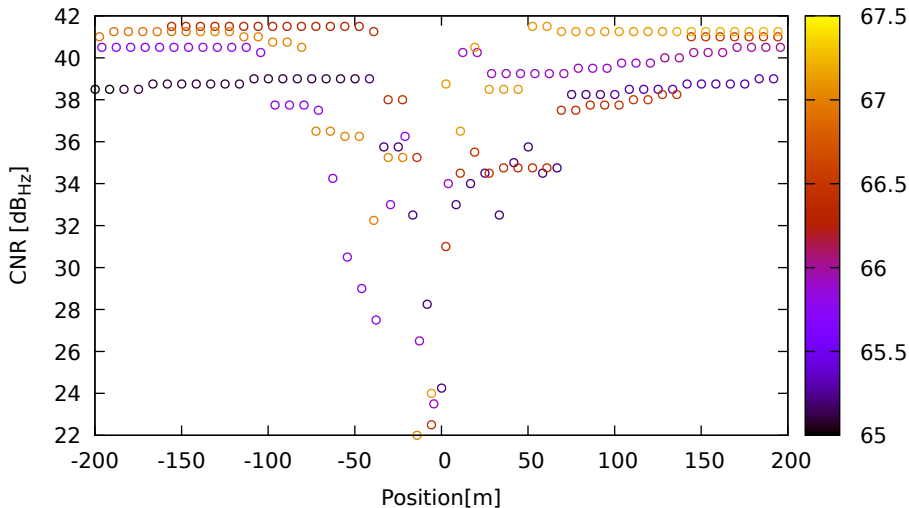
CNR vs position for E10 (E1) on Xiaomi11T - DOY 263 jam. 2
