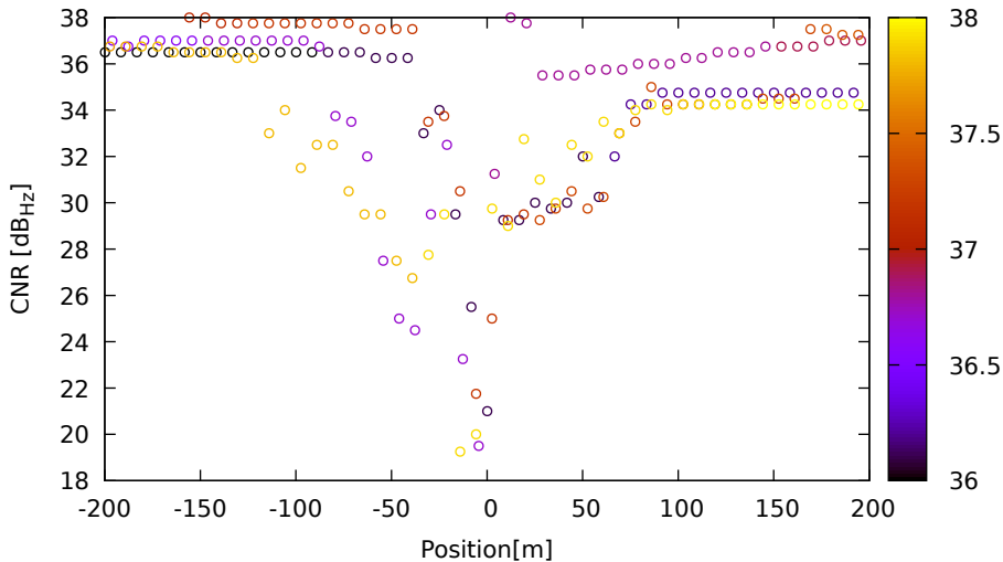
CNR vs position for E11 (E1) on Xiaomi11T - DOY 263 jam. 2
