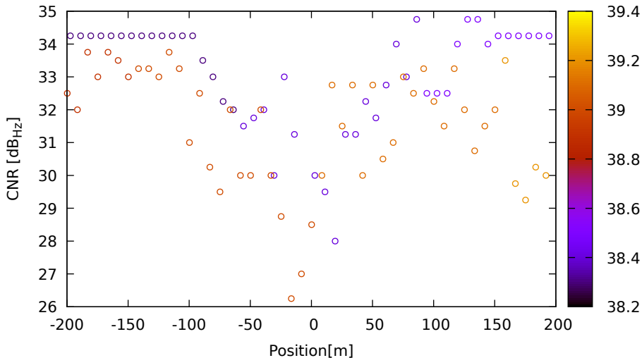
CNR vs position for E11 (E1) on Xiaomi11T - DOY 263 jam. 3
