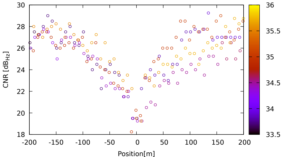
CNR vs position for E11 (E5a) on Xiaomi11T - DOY 263 jam. 1
