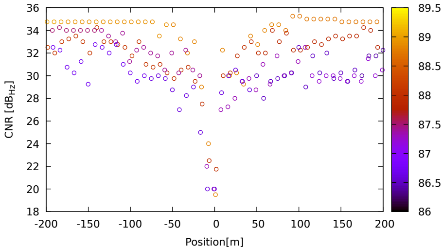
CNR vs position for E12 (E1) on Xiaomi11T - DOY 263 jam. 1
