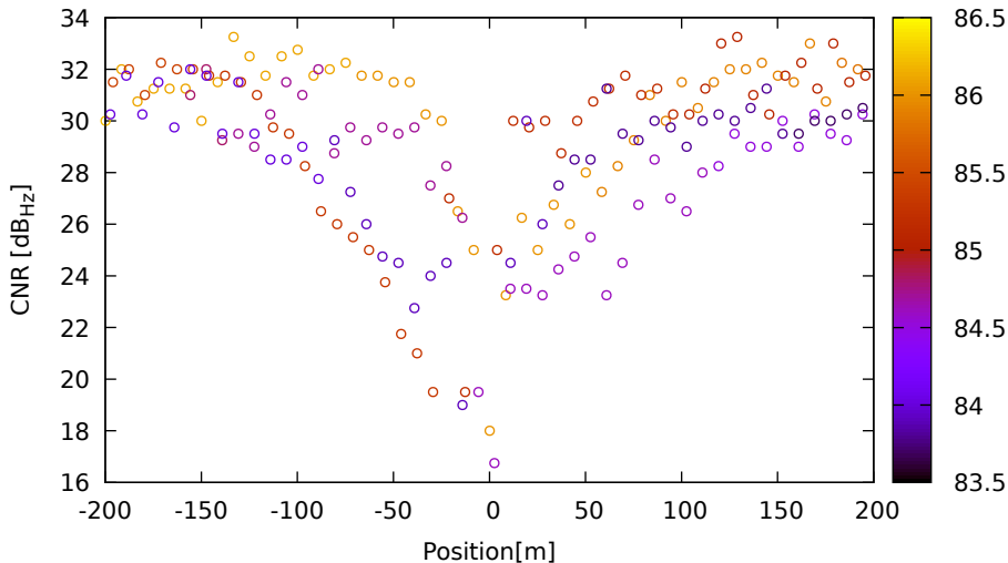
CNR vs position for E12 (E1) on Xiaomi11T - DOY 263 jam. 2
