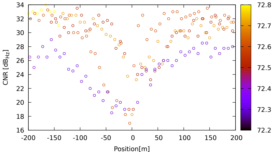
CNR vs position for E19 (E1) on Xiaomi11T - DOY 263 jam. 2
