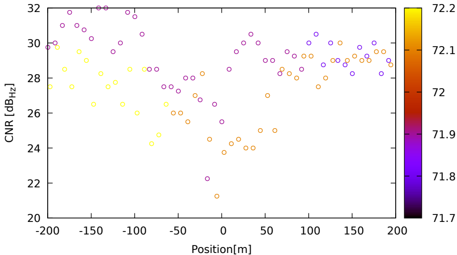
CNR vs position for E19 (E1) on Xiaomi11T - DOY 263 jam. 3
