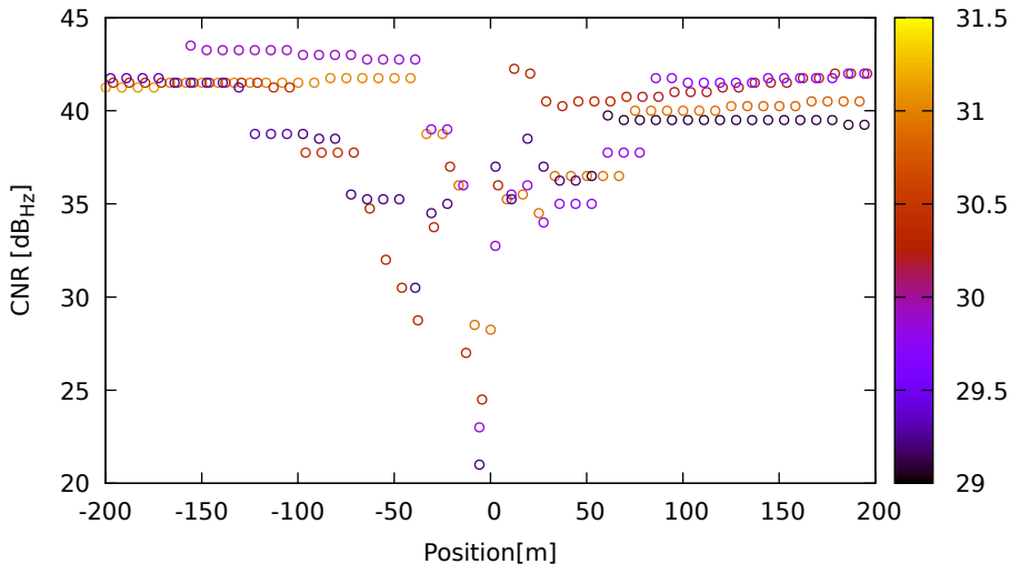
CNR vs position for E33 (E1) on Xiaomi11T - DOY 263 jam. 2
