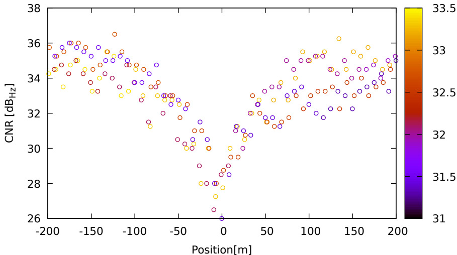
CNR vs position for E33 (E5a) on Xiaomi11T - DOY 263 jam. 1
