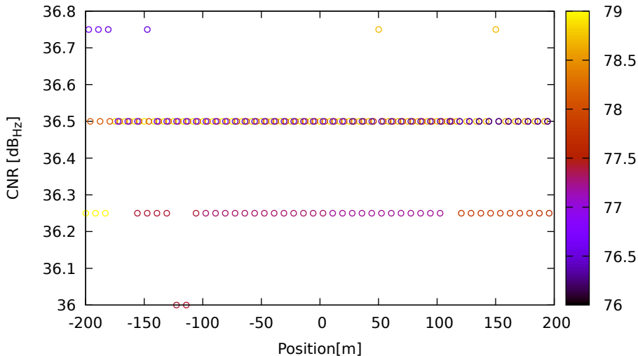
CNR vs position for G01 (L5) on Xiaomi11T - DOY 263 jam. 2
