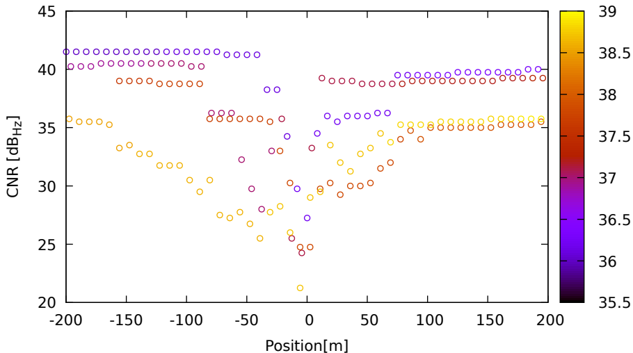
CNR vs position for G04 (L1) on Xiaomi11T - DOY 263 jam. 2
