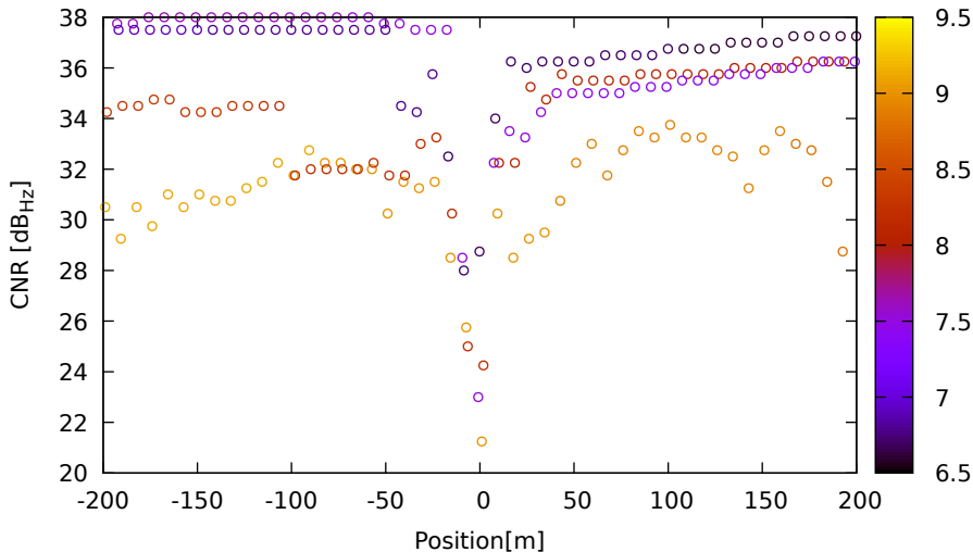
CNR vs position for G08 (L1) on Xiaomi11T - DOY 263 jam. 1
