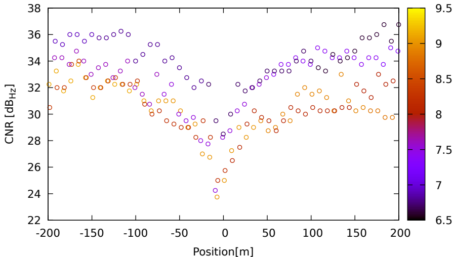
CNR vs position for G08 (L5) on Xiaomi11T - DOY 263 jam. 1
