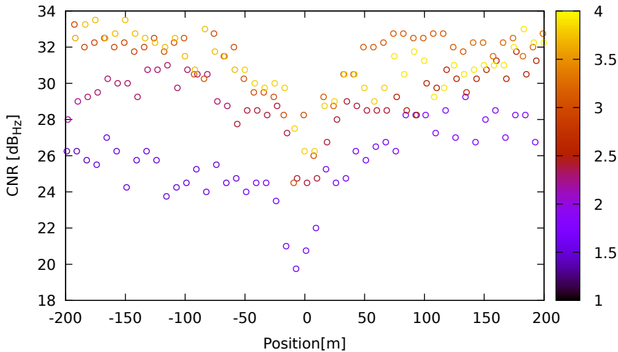
CNR vs position for G09 (L5) on Xiaomi11T - DOY 263 jam. 1
