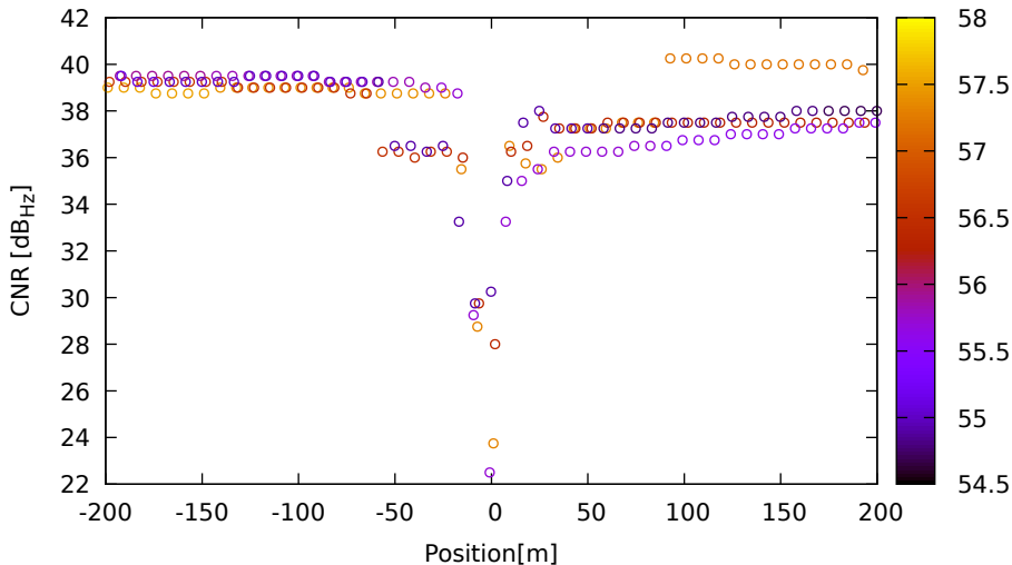
CNR vs position for G21 (L1) on Xiaomi11T - DOY 263 jam. 1
